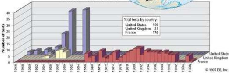
Pacific nuclear tests 1946 to 1996
