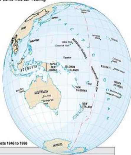
Pacific Nuclear Testing
